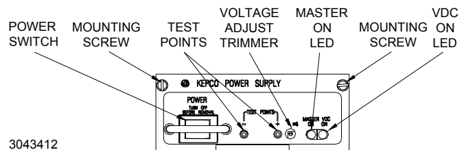
FIGURE 6. COMPONENT LOCATIONS
