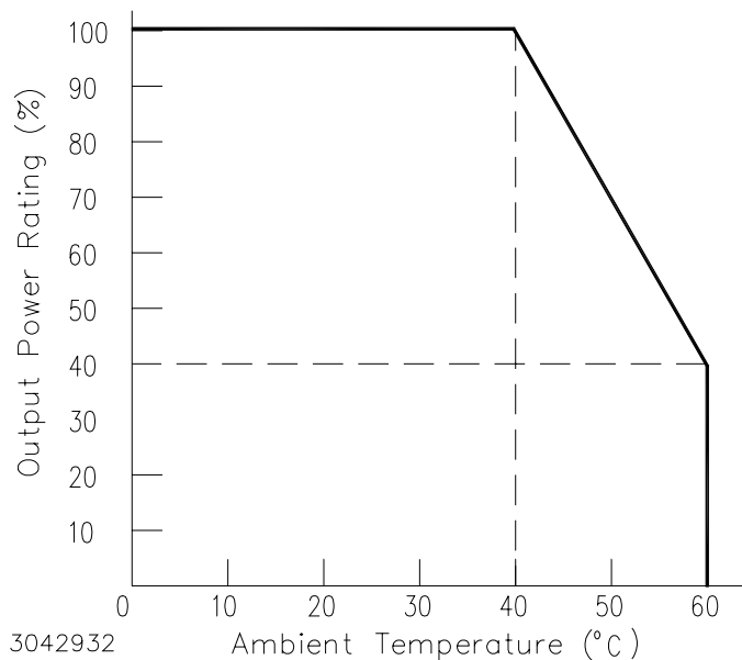
FIGURE 5. % OUTPUT POWER RATING VS. AMBIENT TEMPERATURE
