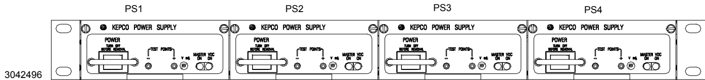
FIGURE 2. HSF-1UR 50 WATT POWER SUPPLIES (4) INSTALLED IN RA 19-1U RACK ADAPTER
