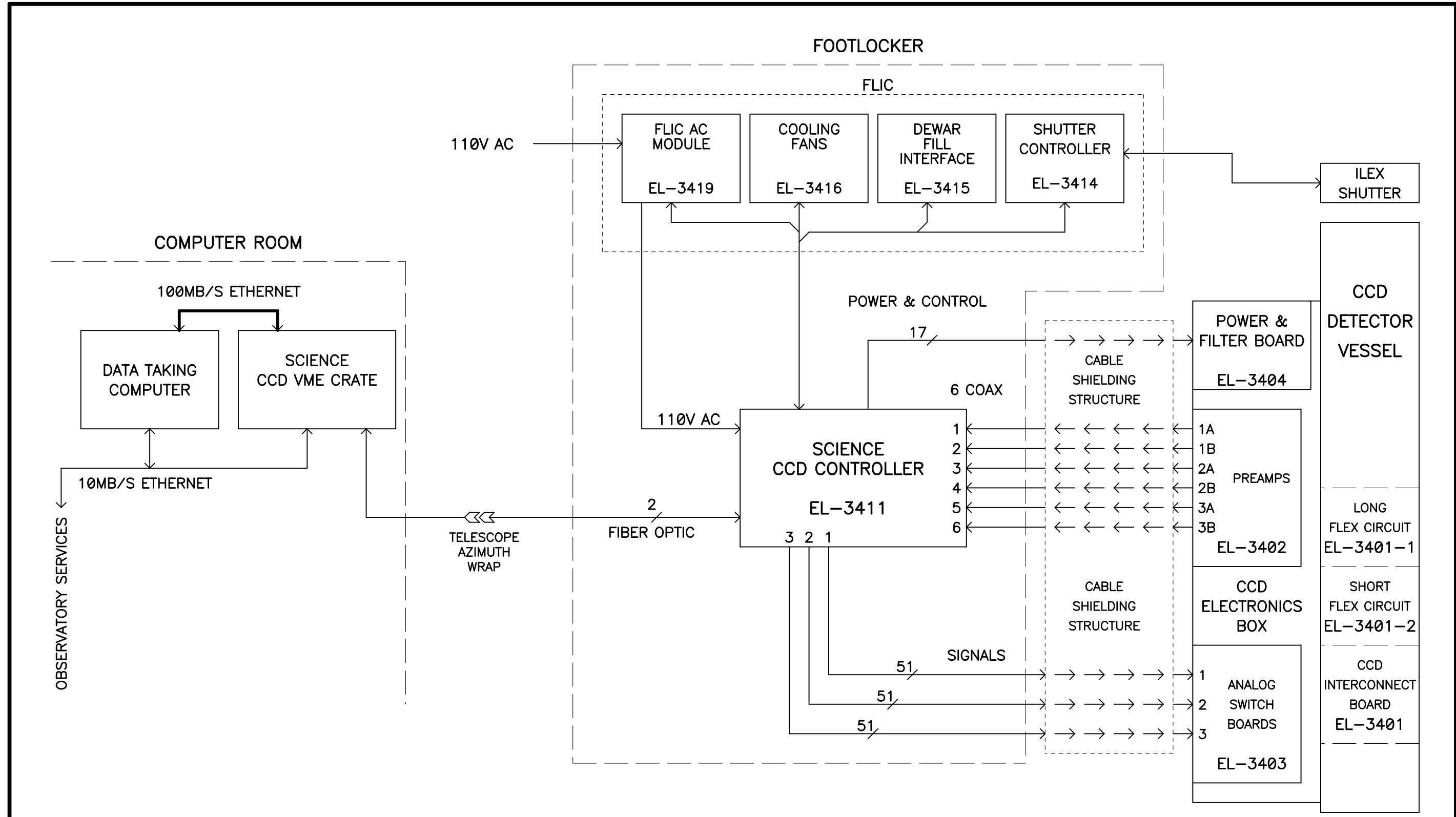
Block Diagram HIRES CCD Upgrade
